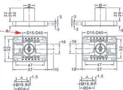
Lock Housing 21-206-8
